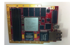
FMC667 C6678 FMC Card
